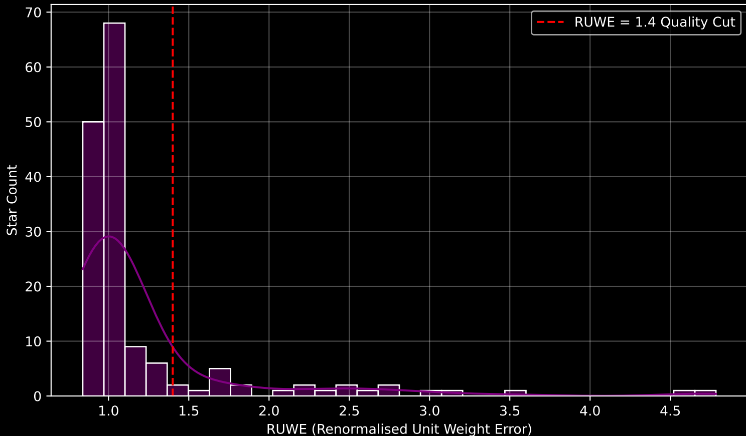
GAPOGEE DR17 Field [223+26_MGA] RUWE Distribution (n= 157)
