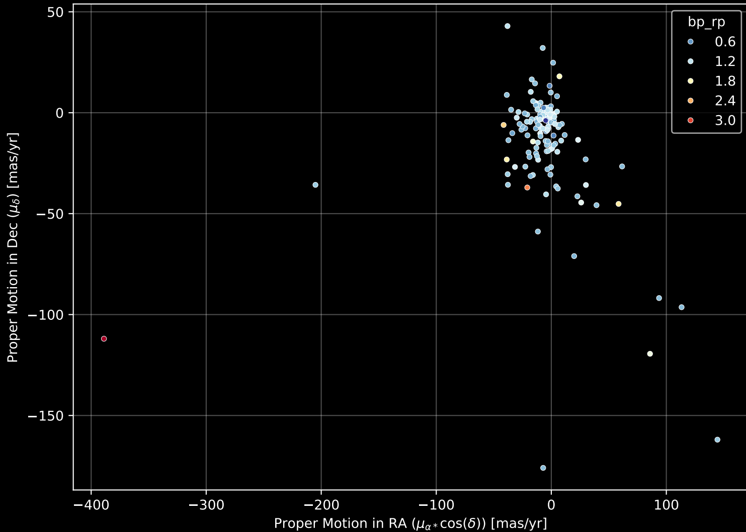
APOGEE DR17 Field: [223+26_MGA] Proper Motion Diagram (n= 166)
