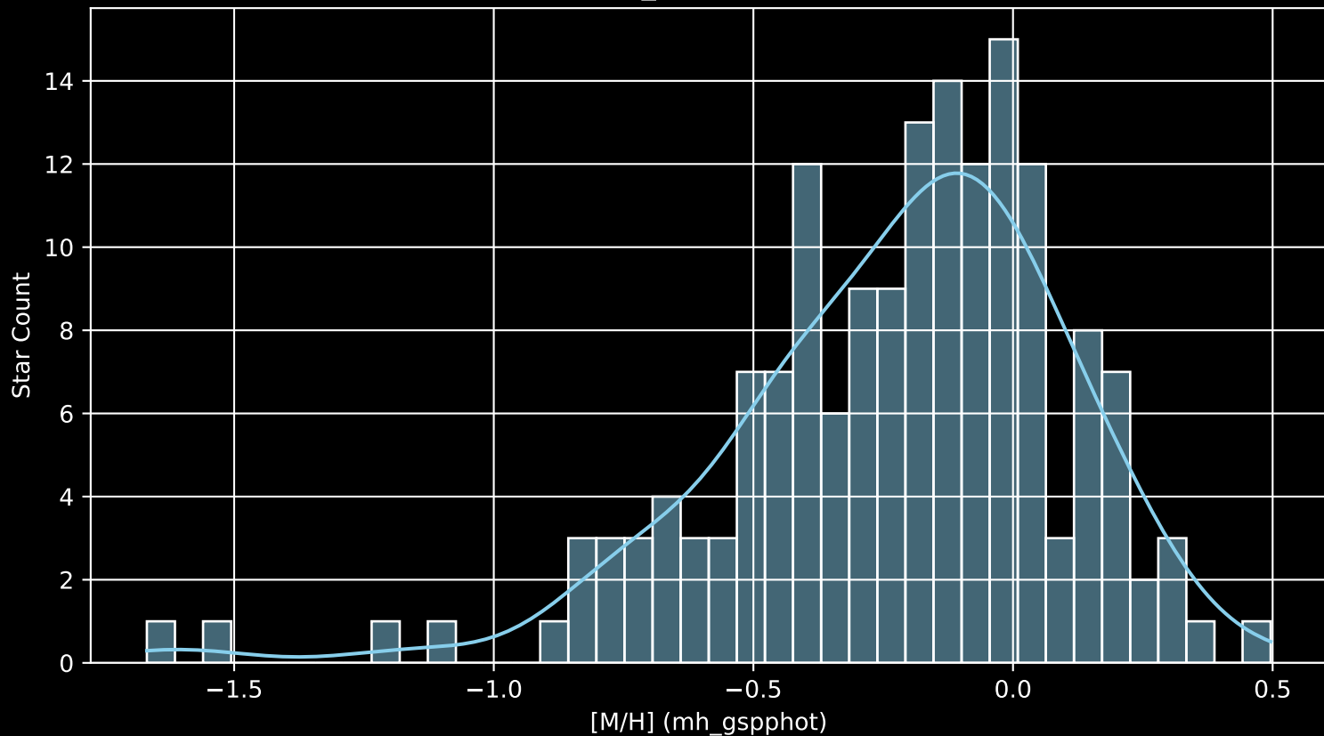
APOGEE DR17 Field: [223+26_MGA [M/H] (mh_gspphot) (n= 165)
