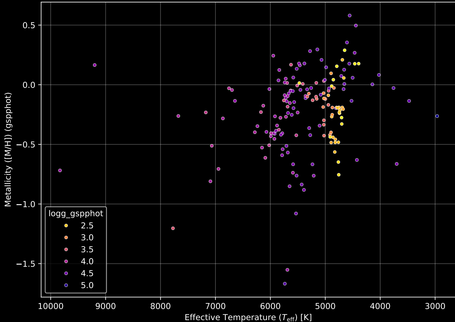
APOGEE DR17 Field: [223+26_MGA] Stellar Population Parameters (n= 166)
