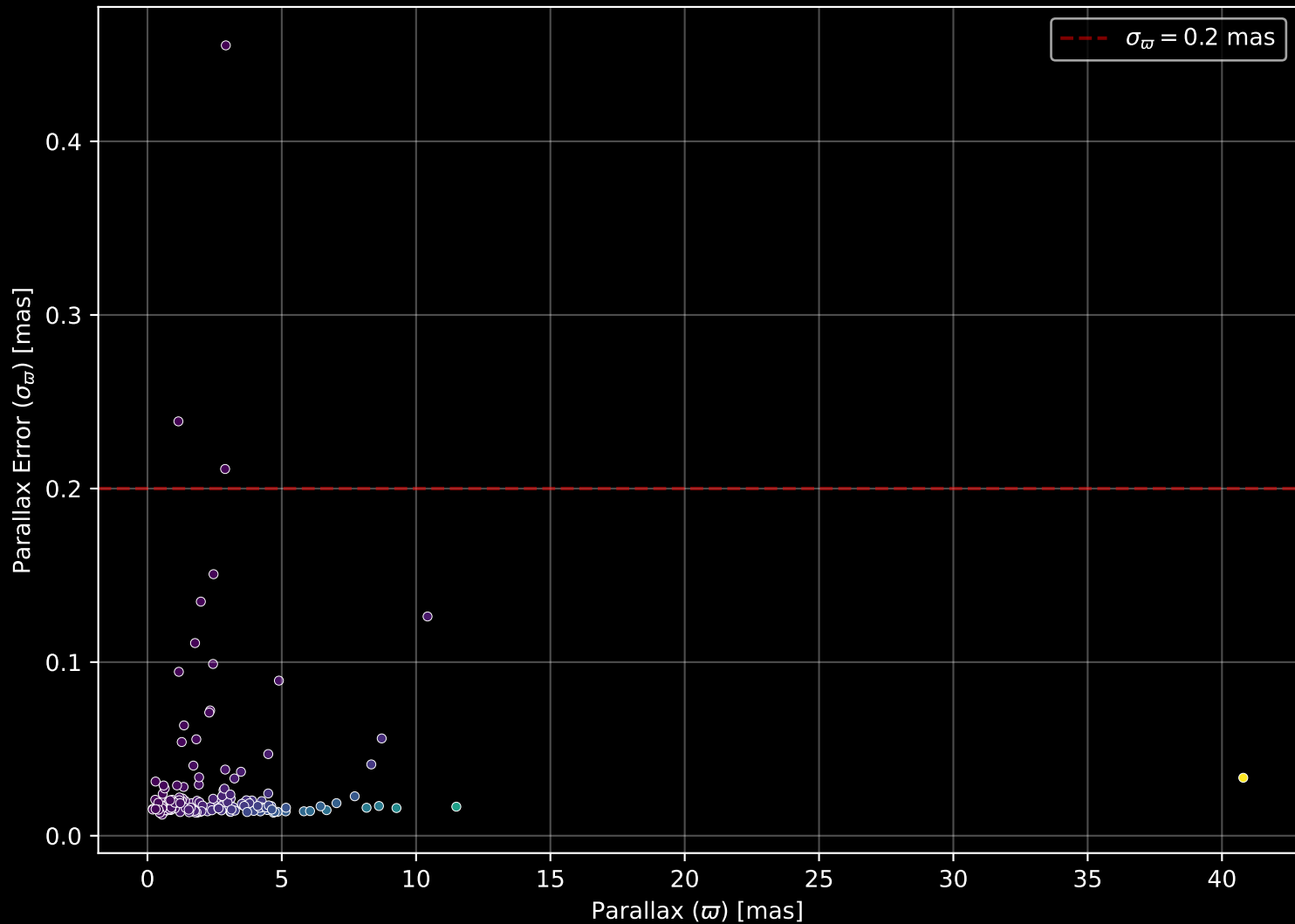
APOGEE DR17 Field: [223+26_MGA] Parallax Quality (n= 166)
