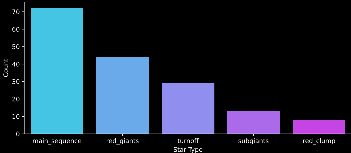
APOGEE DR17 Field: [223+26_MGA] Count plot of Star Type
